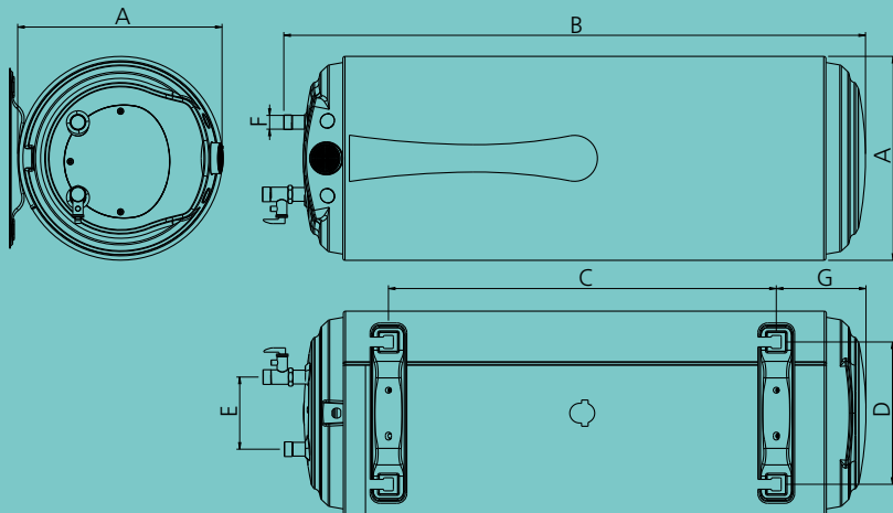
Left hand side inlet outlet
