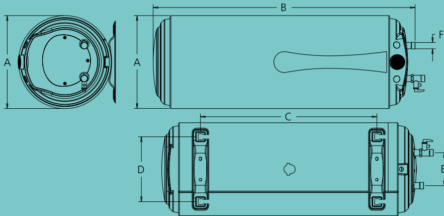
Right hand side inlet outlet
